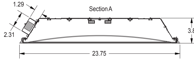
End Profile with Driver Box
