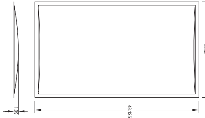
Diffuser Dimensions
