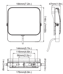
90W&120W(Yoke Mount)
