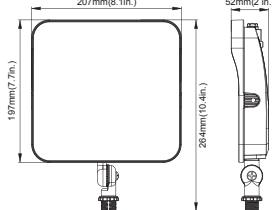
40W&65W(Knuckle Mount)
