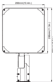
90W&120W(Slipfitter Mount)
