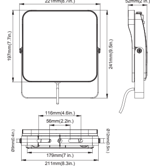
40W&65W(Trunnion Mount)
