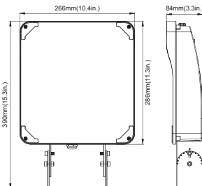
90W&120W(Yoke Mount)
