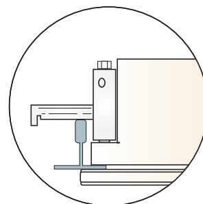
OVERLAP DOOR GRID CEILING
