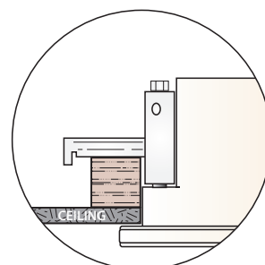
OVERLAP DOOR RECESSED CEILING
