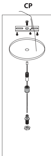
Cord Pendant (No Power Feed)
