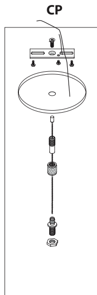
Cord Pendant (No Power Feed)
