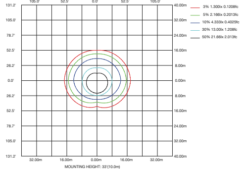
ISOLUX DIAGRAM
