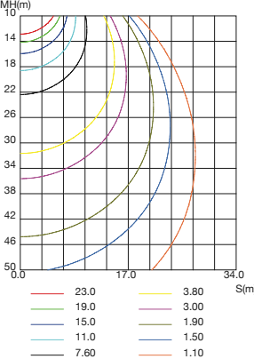
C0 PLANE ISOLUX DIAGRAM (UNIT:lx)
