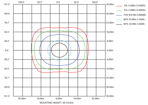
ISOLUX DIAGRAM
