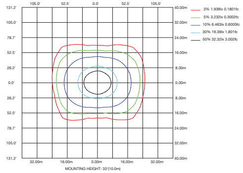
ISOLUX DIAGRAM
