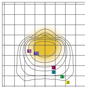
ARL680-445W-T4 Mounting Height=25.00 FT
