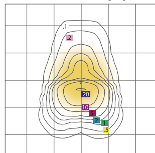
ARL680-540W-AT4 Mounting Height=30.00 FT
