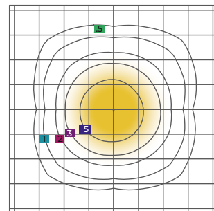
ARL680-445W-T5 Mounting Height=25.00 FT
