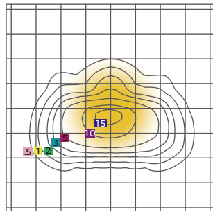
ARL680-445W-T3 Mounting Height=30.00 FT
