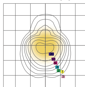
ARL680-540W-AT6 Mounting Height=25.00 FT
